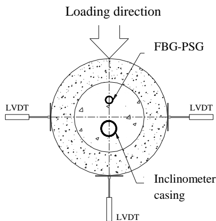
Figure 2. Positions of FBG-PSG and inclinometer casing.
